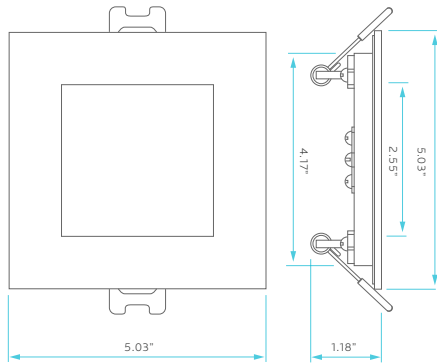
CUTOUT: Ø 4.25"
